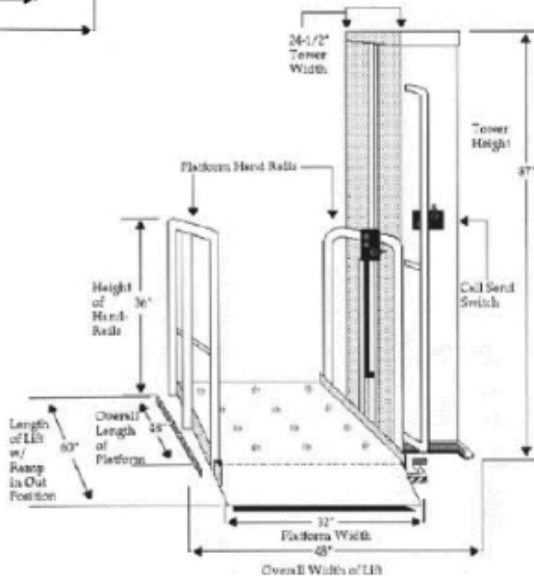
Right: HPL72 Schematic Drawing
