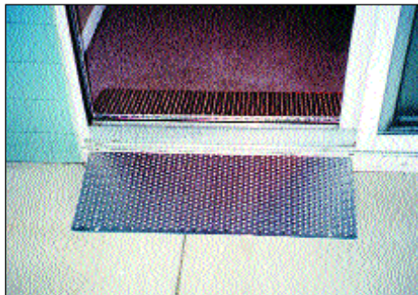
Left: The Patio Doorway Threshold Ramp. Inside: One-inch rise made accessible with the TR1 model. Outside: Three-inch rise made accessible with the TR3 model.
